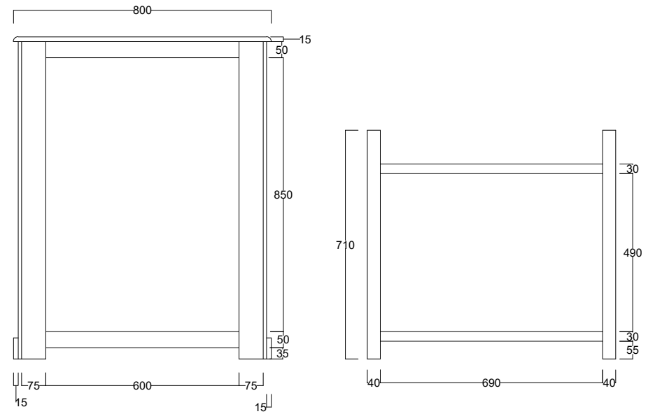
BACK VIEW
